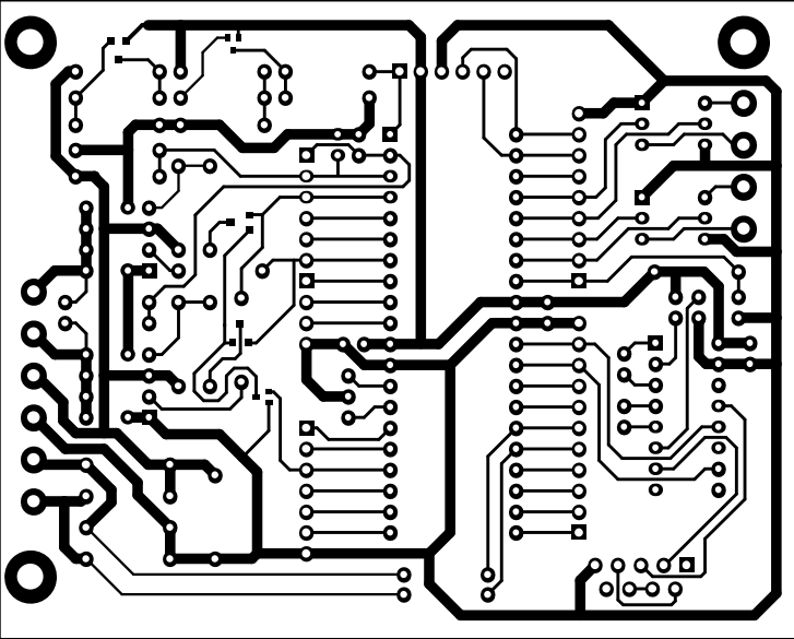
Bottom Layer print, as seen from top layer (ie through board)
